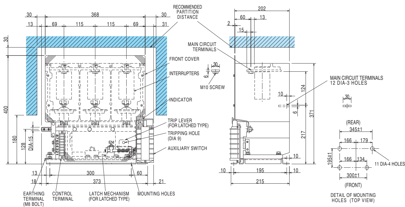
Fig. 4 Types CV-6HA(L)-2
