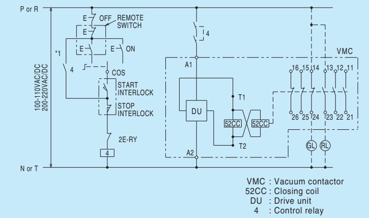
Fig. 10 Non-Latched type operating circuit
