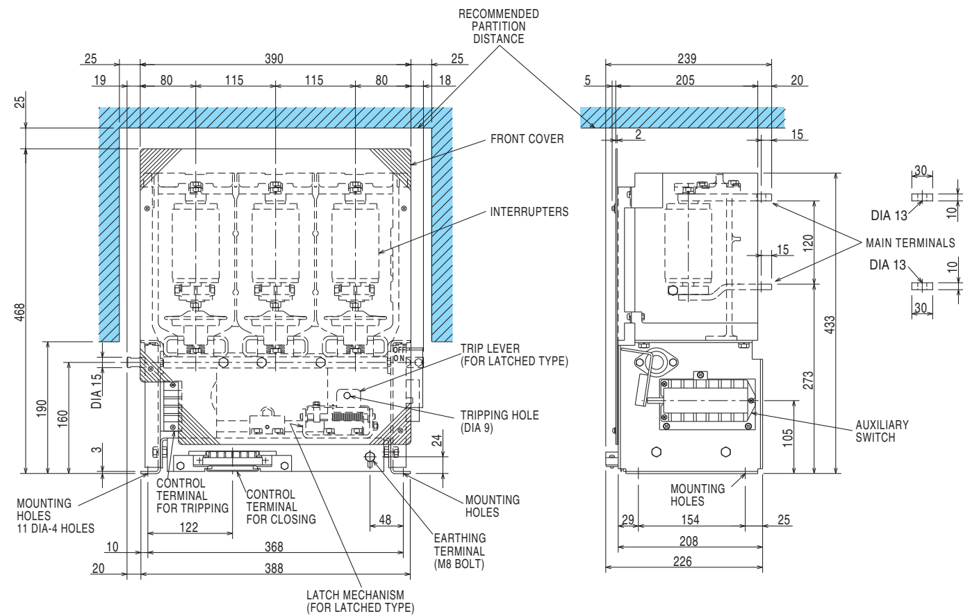
Fig. 8 Types CV-6KA1/CV-6KAL1
