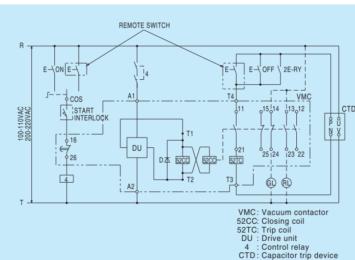
Fig. 12 Latched type operating circuit (Capacitor trip)
