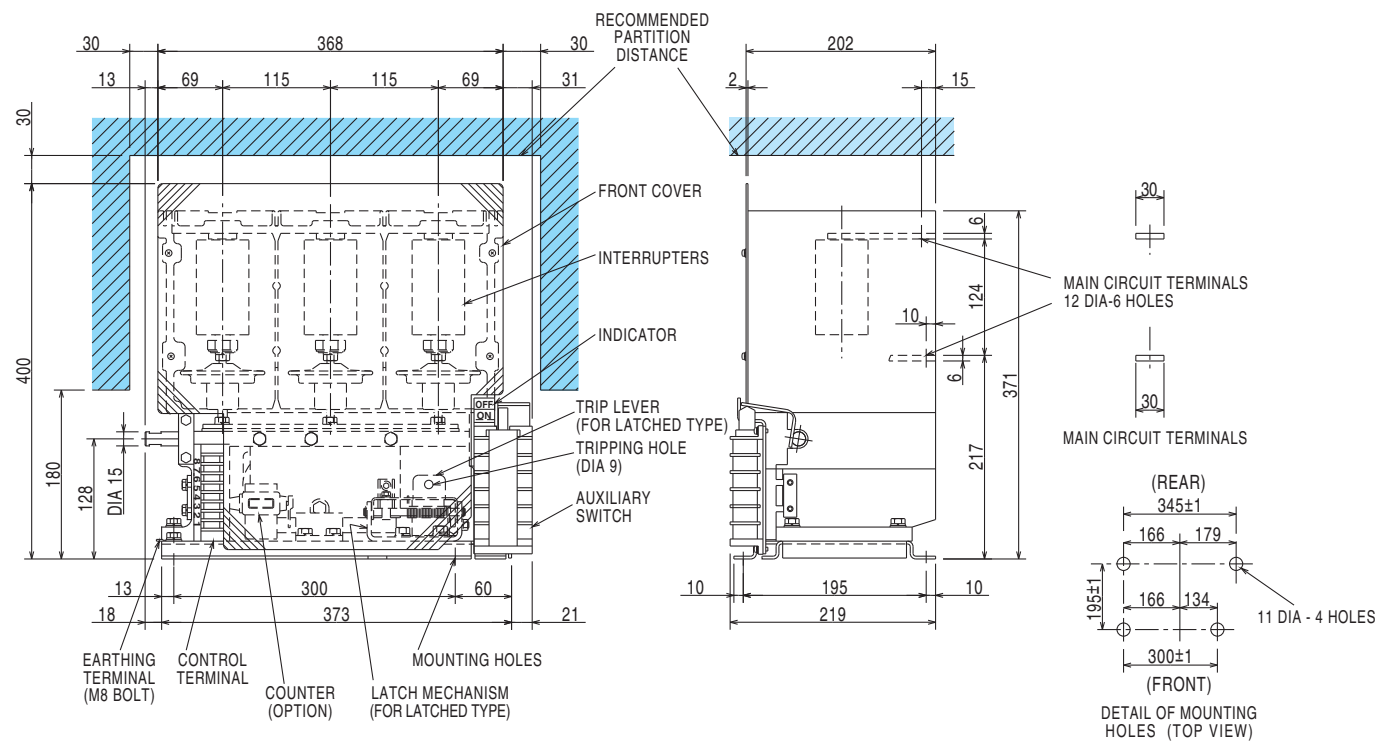
Fig. 3 Types CV-6GA(L)/CV-6HA(L)
