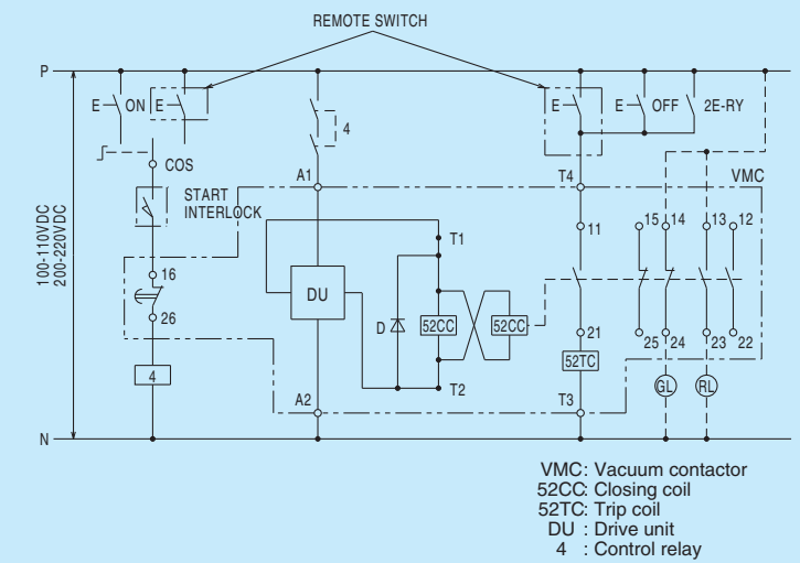
Fig. 11 Latched type operating circuit (Shunt trip)
